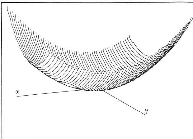
Figure 7: A Quadratic Surface
