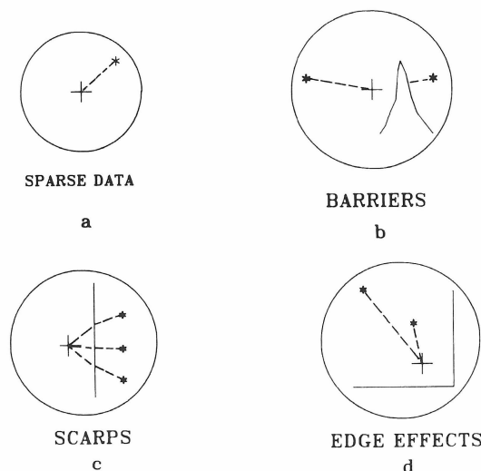
Figure 3: Neighbourhood Problems
