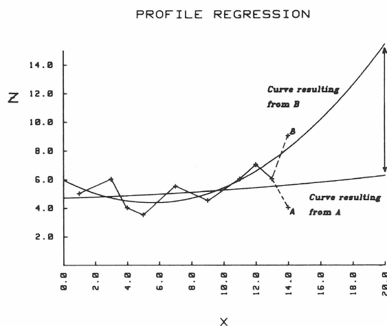
Figure 9: Problems in Extrapolation
