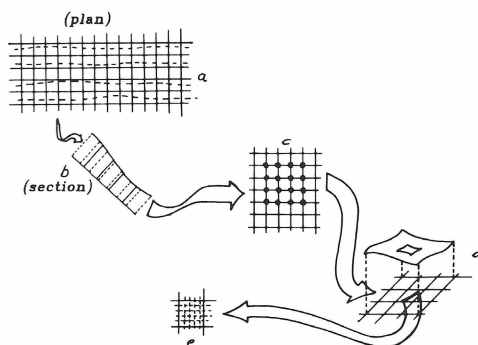
Figure 14: The HCS Interpolation Scheme
