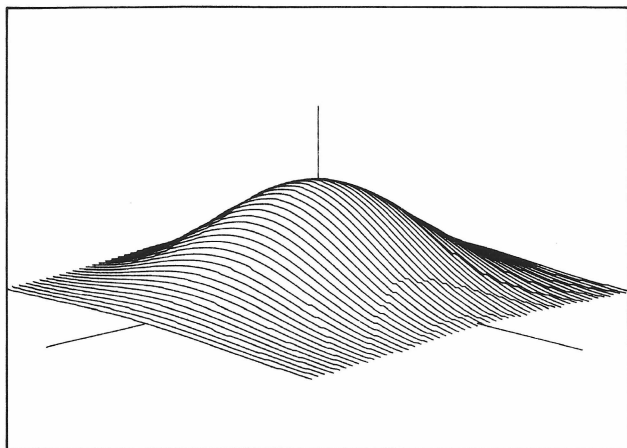
Figure 5: An Exponential Surface
