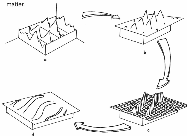
Figure 1: Interpolation and Contouring
