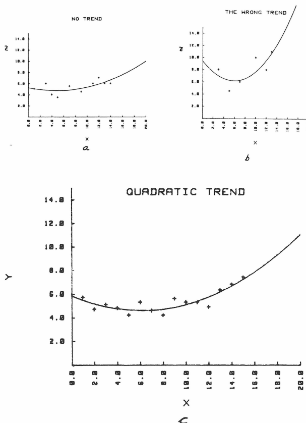
Figure 8: Trend Fitting
