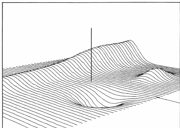
Figure 6: A Fourier Surface
