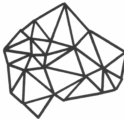
Figure 10: A Triangular Irregular Network
