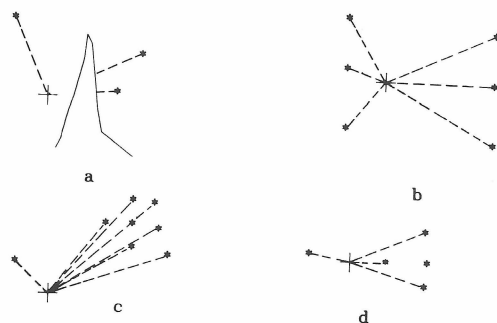
Figure 4: Weighting Problems
