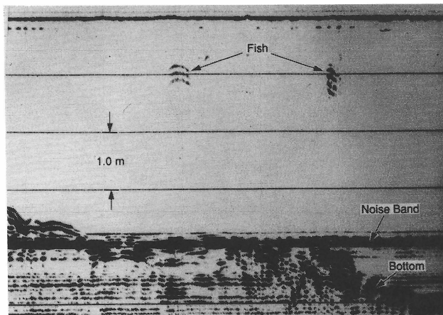
Figure 7: Fish targets in the radar profile taken near Grass Island, where several "fishermen" were at work.
