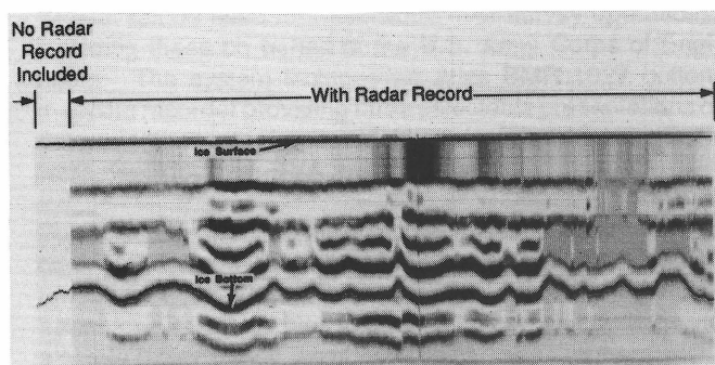
Figure 9: Radar record of snow-free sea ice, approximately 1.7 m thick.
