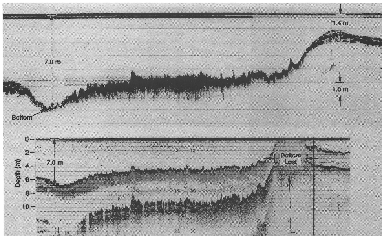
Figure 3: Radar (top) and sonar (bottom) profiles obtained in the Grass River
