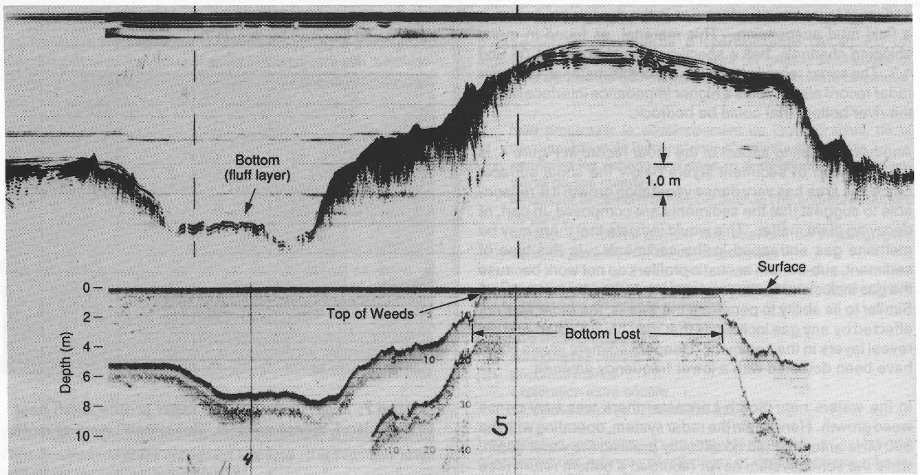
Figure 4: Radar (top) and sonar (bottom) profiles obtained off Grass Island
