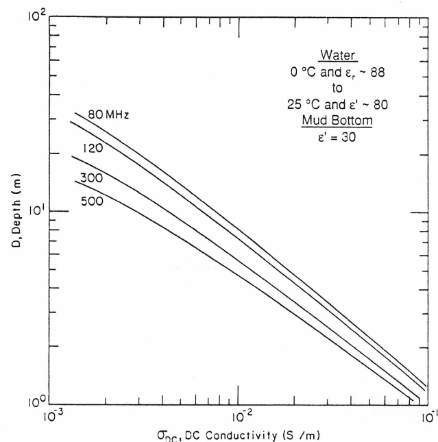
Figure 1: Estimated impulse radar profiling depth versus water conductivity with transmitted wavelet center frequency in water as a parameter
