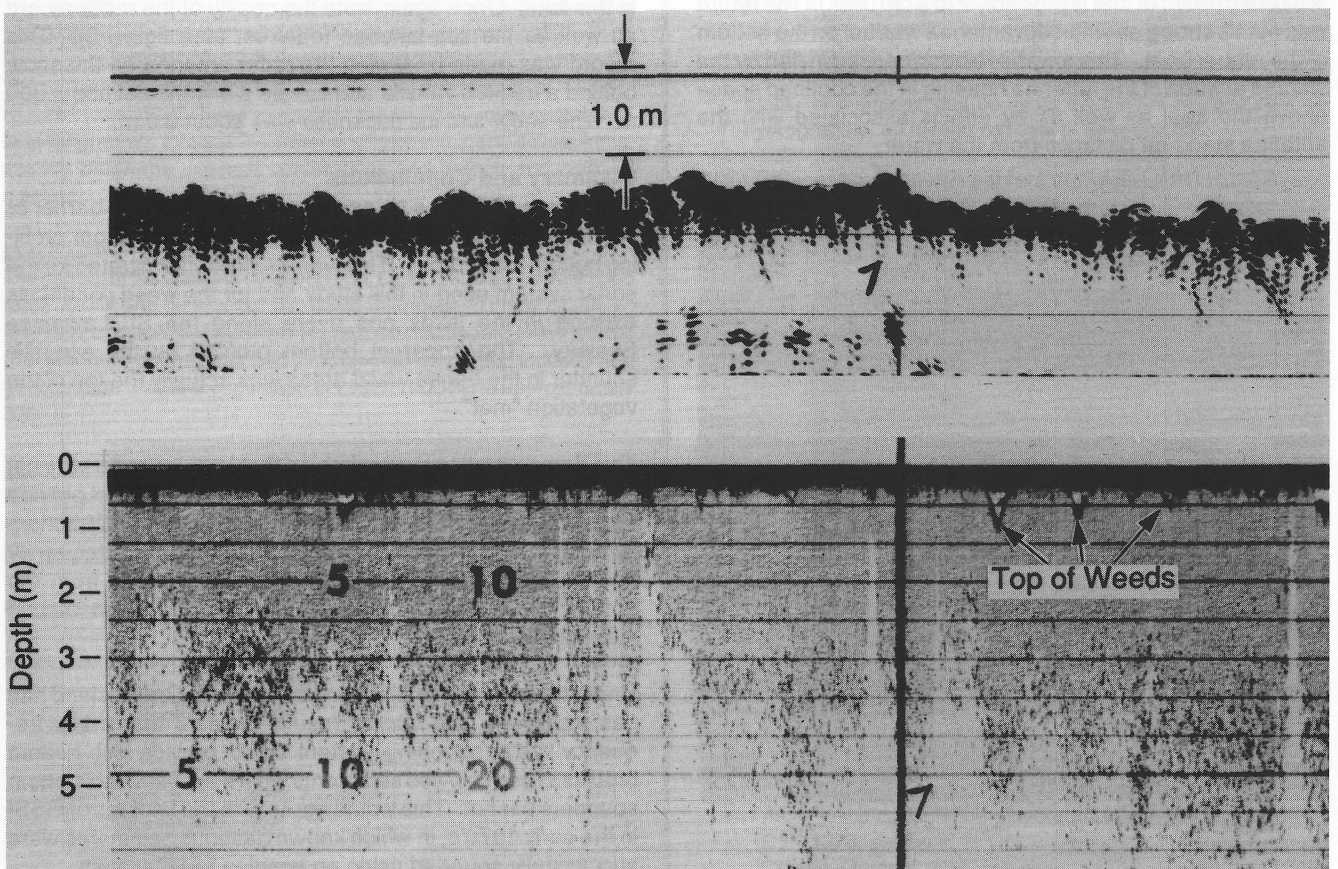
Figure 5: Radar (top) and sonar (bottom) profiles obtained on the north side of Lake St. Francis near South Lancaster
