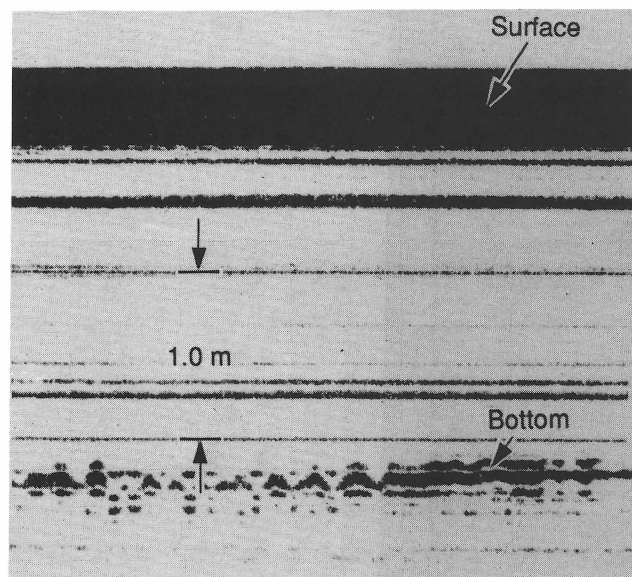
Figure 6: A through-hull bottom profile made with a 500 MHz antenna. The water is about 2.2 m deep.
