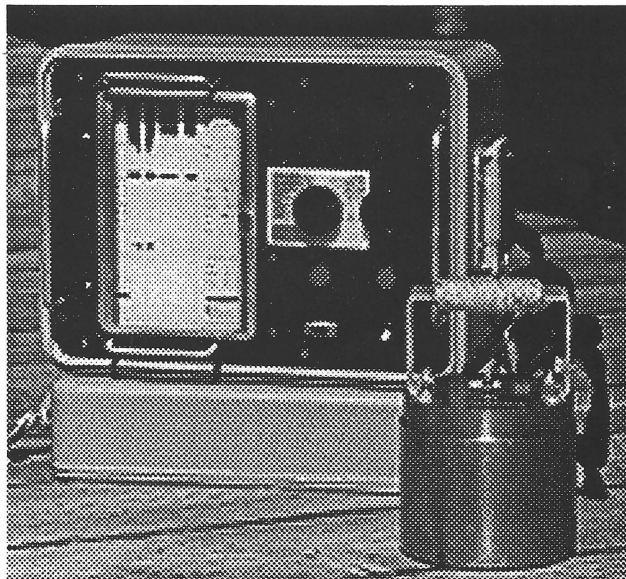
Figure 1: The KEL 320A Arctic Sounder
