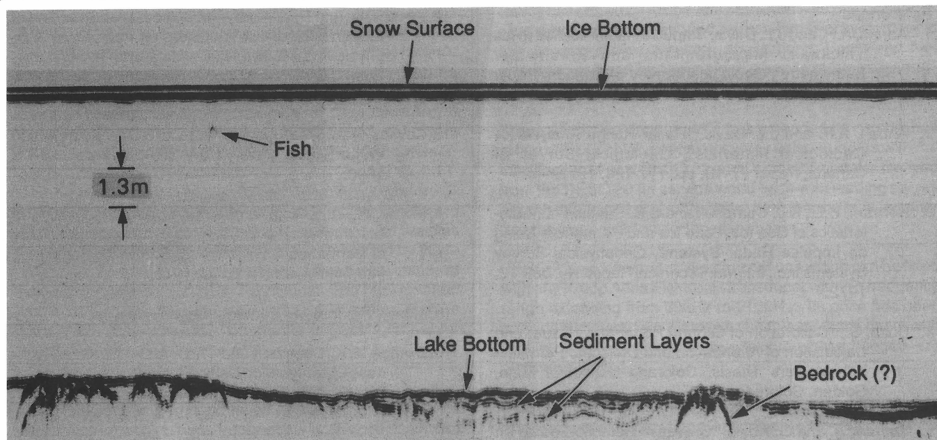
Figure 8: Radar record showing the snow thickness, ice thickness and bathymetry at a Lake Nipissing site.
