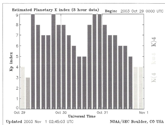
Figure 2: Kp values for October 29-31, 2003 (NOAA SEC)
