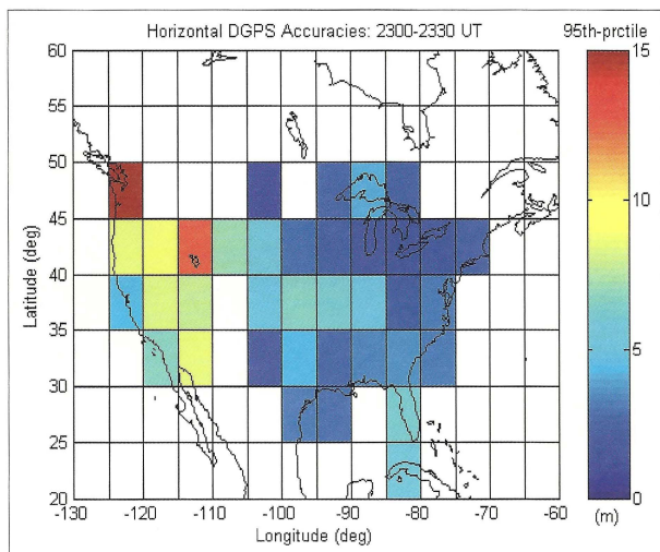
Figure 6: 95th-percentile DGPS horizontal positioning accuracies for the period 23:00-23:30 UT October 30, 2003, for baselines of lengths 100-200km.
