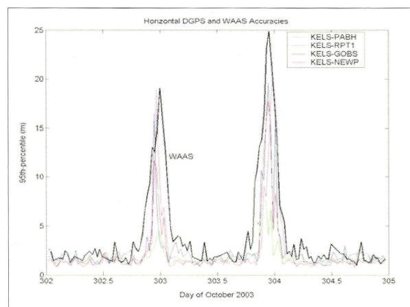
Figure 8: 95th-percentile DGPS and WAAS horizontal positioning accuracies for October 29 (day 302) - 31 (day 304), 2003. User KELS is located in the northwest United States.
