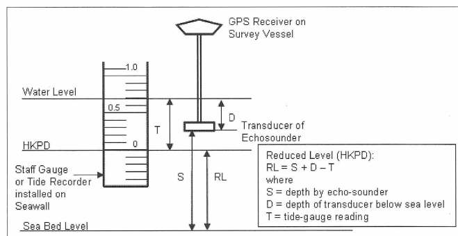
Figure 2: Reduction of soundings from tide-gauge readings
