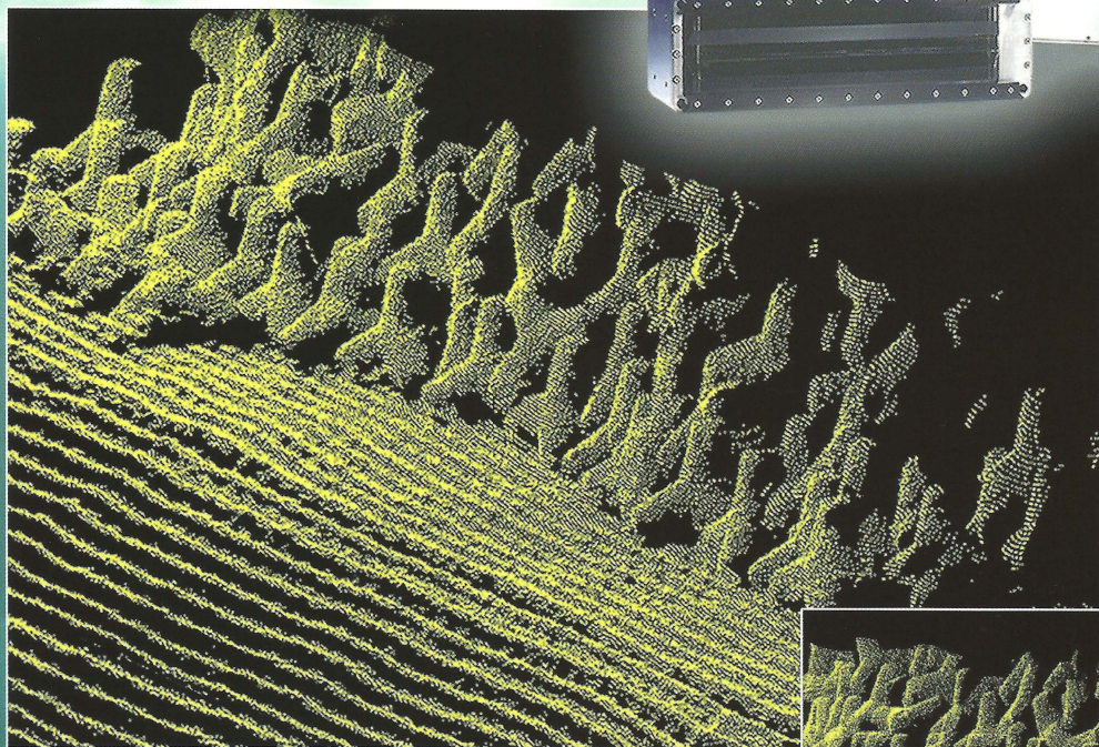
Individual SeaBat 8125 soundings of Breakwater Tetrapodes, courtesy of Nihon Zitan, Japan
