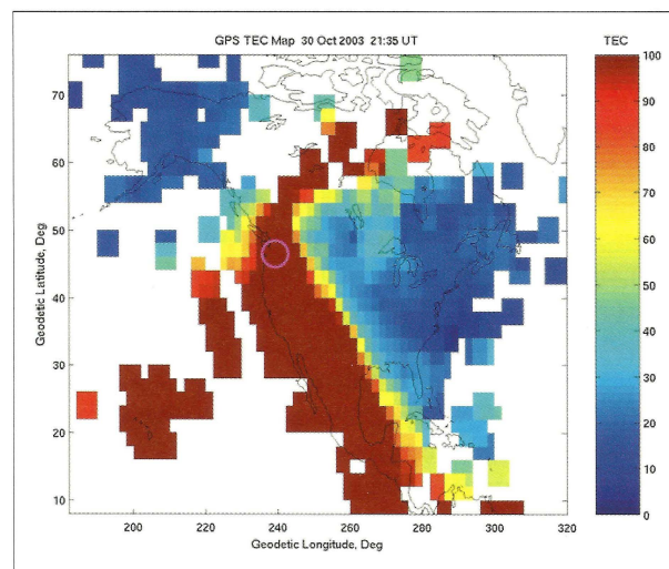
Figure 3: Storm enhanced density effect shown in TEC map (units are TECU) derived from more than 400 GPS reference stations (21:35 UT, October 30, 2003). The light coloured circle indicates a region of large ionosphere gradients.
