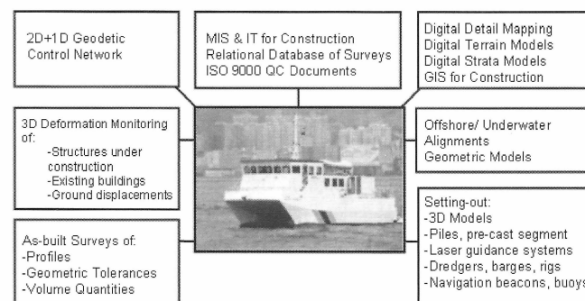
Figure 1: Survey operations for coast construction projects (Lam, 2005)
