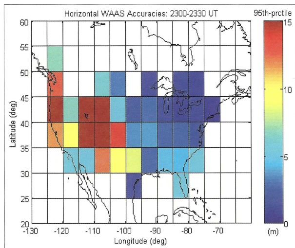
Figure 7: 95th-percentile WAAS horizontal positioning accuracies for the period 23:00-23:30 UT October 30, 2003.
