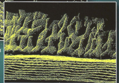
Individual SeaBat 8125 soundings of Breakwater Tetrapodes, courtesy of Nihon Zitan, Japan
