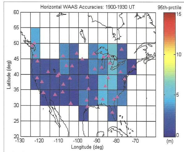
Figure 5: 95th-percentile WAAS horizontal positioning accuracies for the period 19:00-19:30 UT October 30, 2003. Locations of CORS reference stations used in the processing are shown as triangles.
