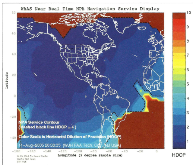
Figure 1: WAAS horizontal positioning coverage (FAA, 2005)
