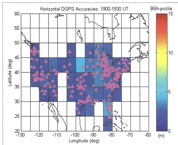
Figure 4: 95th-percentile DGPS horizontal positioning accuracies for the period 19:00-19:30 UT October 30, 2003, for baselines of lengths 100-200km. Locations of CORS reference stations used in the DGPS processing are shown as triangles.
